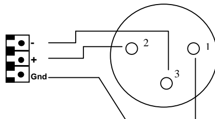
Balanced line → XLR Connector
