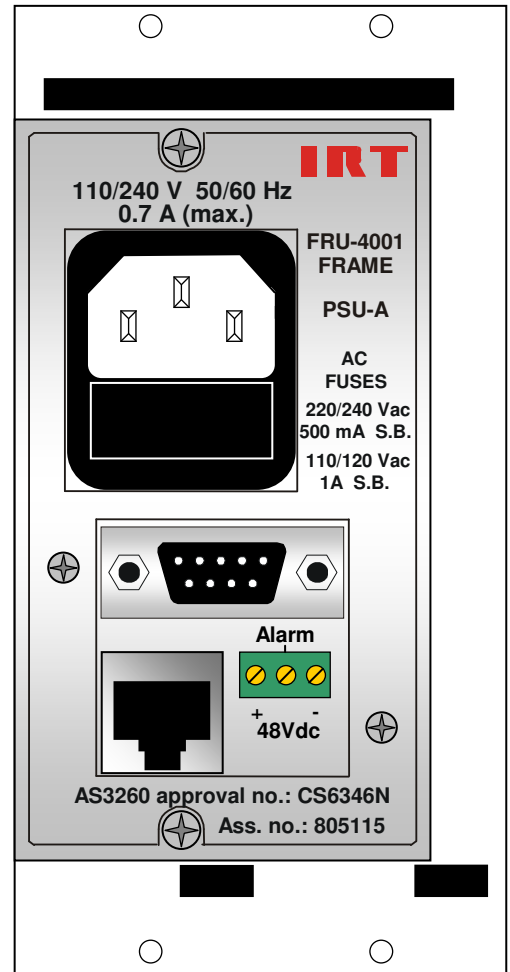
Rear connections on FRU-4001 frame.
